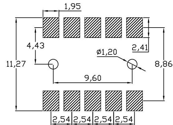
RECOMMENDED PCB LAYOUT TOP VIEW (. XX \pm 0.05 )
